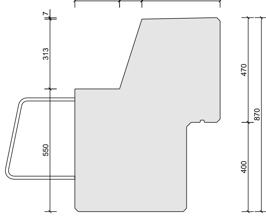
Detail a
