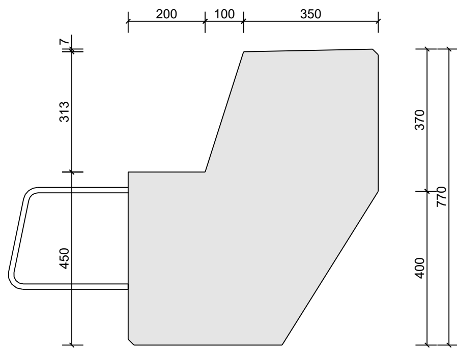
H=450/770
