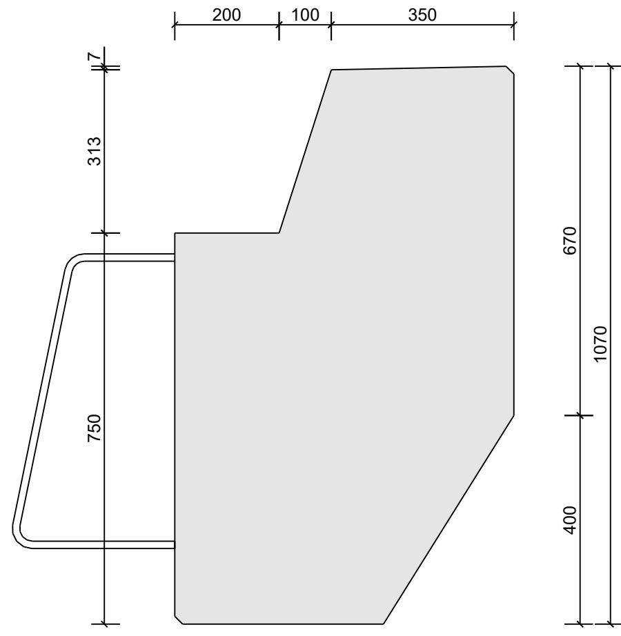
H=750/1070
