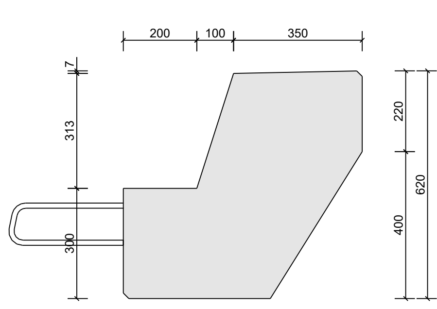
H=300/620
