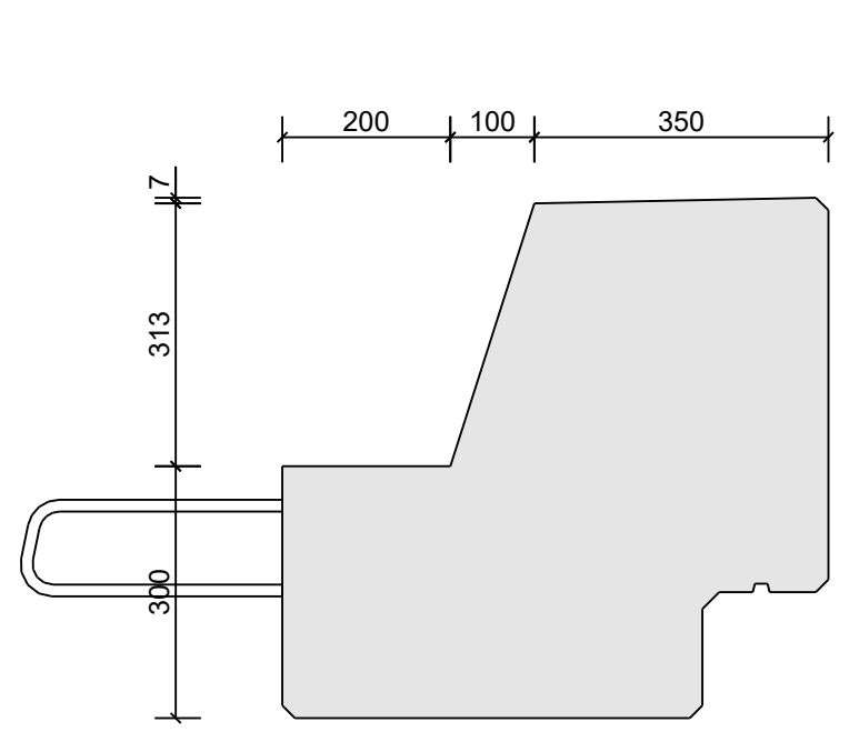
H=300/620
