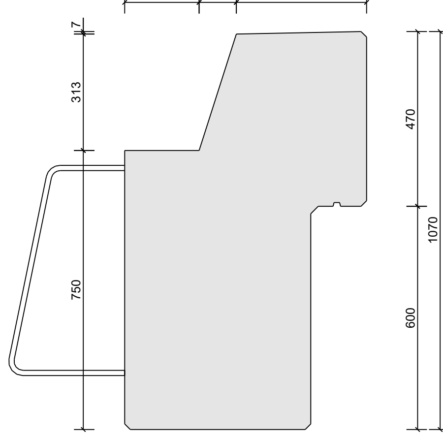
H=750/1070
