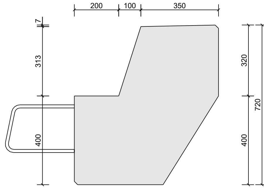
H=400/720
