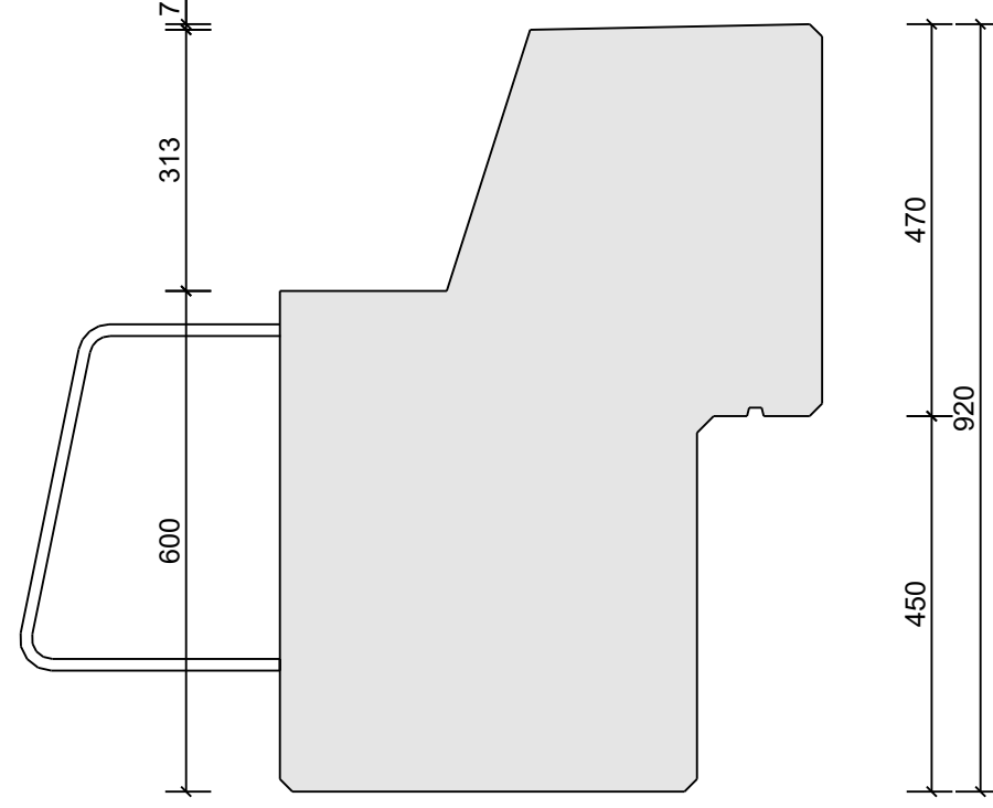
H=600/920
