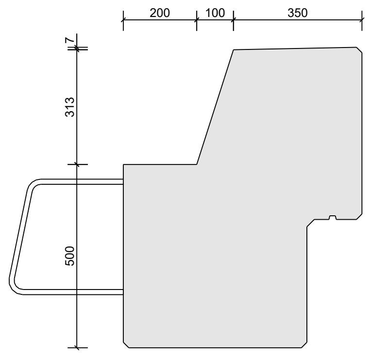
H=500/820
