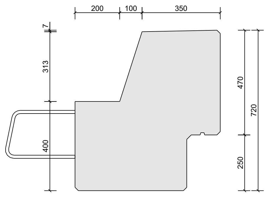
H=400/720
