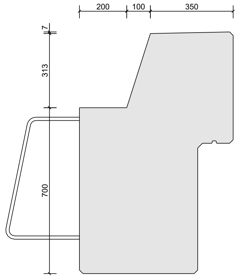
H=700/1020
