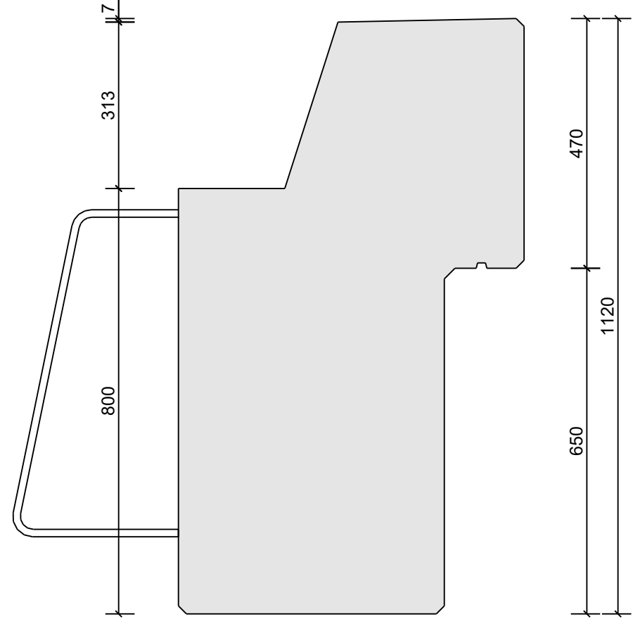
H=800/1120
